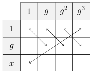
(a) A 3 \times 4 partially matched rectangle. The cyclic closure of (1, 1) spans all rows.
