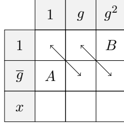
Figure 6: A 3 \times 3 matched rectangle that contains M_3^{\text{cyc}} .
