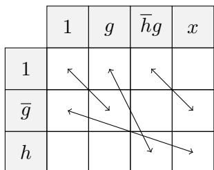
(c) A 3 \times 4 partially matched rectangle. Its core subgroup is isomorphic to BS(1, -1) .
