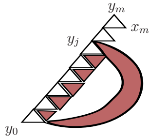
Figure 3: A simple ladder with edges forced by Claim 2.3
