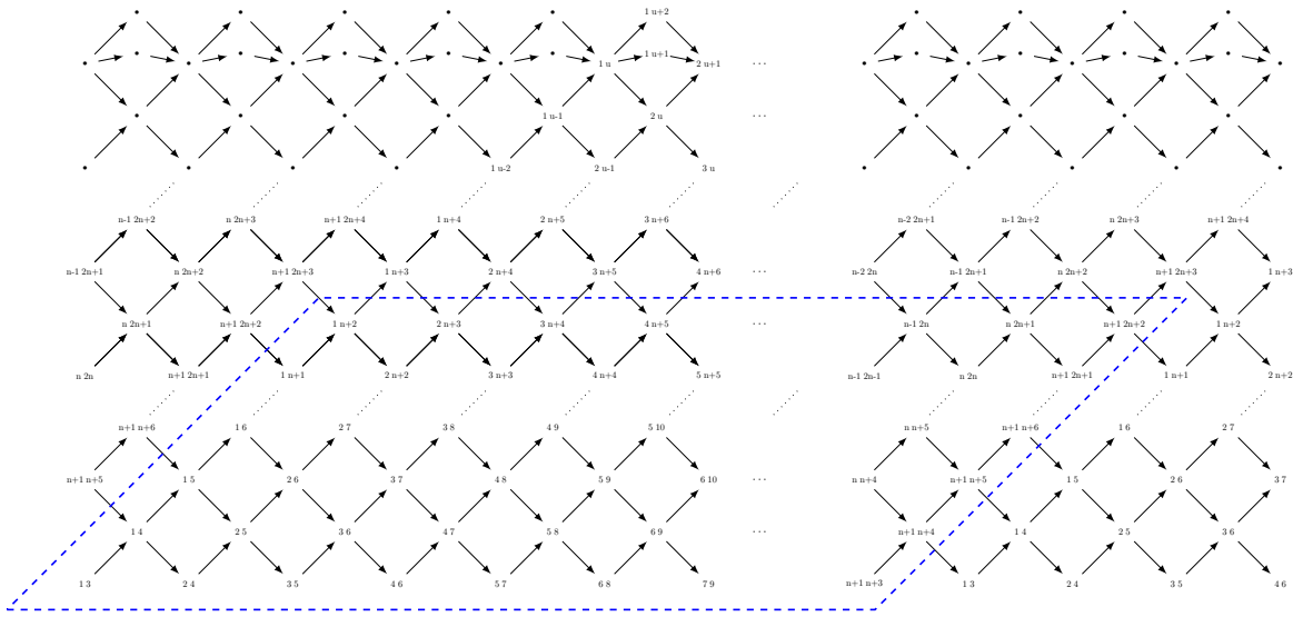
FIGURE 6. The Auslander-Reiten quiver of \mathcal{D}_{n,t} . The objects in \mathcal{R}_{\mathcal{D}_{n,t}} are in the area inside the dashed blue lines. Here u = 2t(n + 1) .
