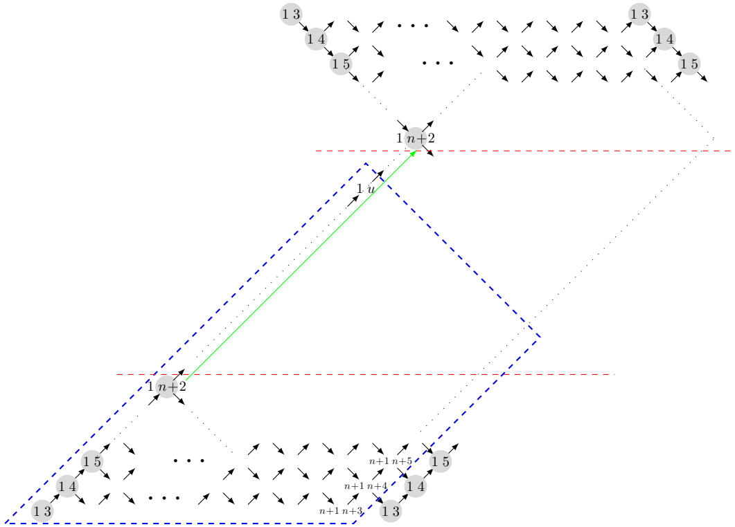
FIGURE 2. A fundamental domain for \mathcal{A}_{n,t} inside the derived category is encircled by a dotted blue line. Below the bottom (and above the top) dotted red line lie all rigid indecomposable objects. The Hom-hammock of (1\ n+2) is emphasized by a dotted rectangle. The green arrow gives rise to a loop in the quiver \mathcal{Q}_{\mathcal{R}_C} . Here u equals (t+1)(n+1) .
