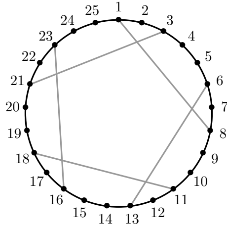
FIGURE 4. A collection of arcs of the icosikaipentagon corresponding to a non-rigid indecomposable object of \mathcal{A}_{4,2} .
