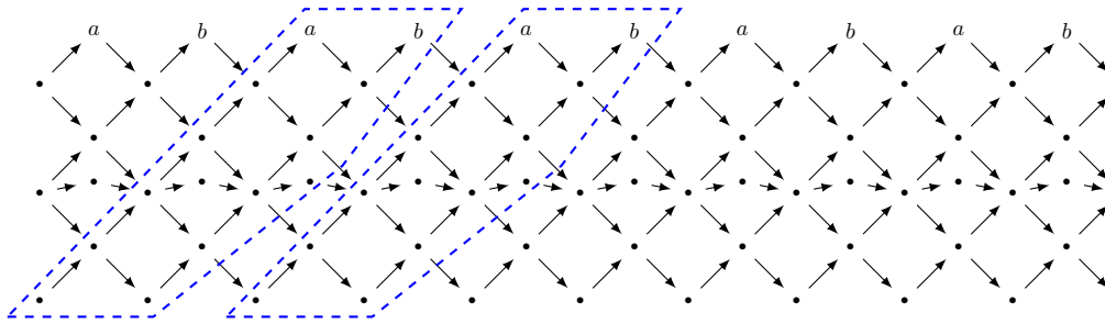
FIGURE 10. The orbit category D^b(\mathbb{K}E_7)/\tau^2 .
