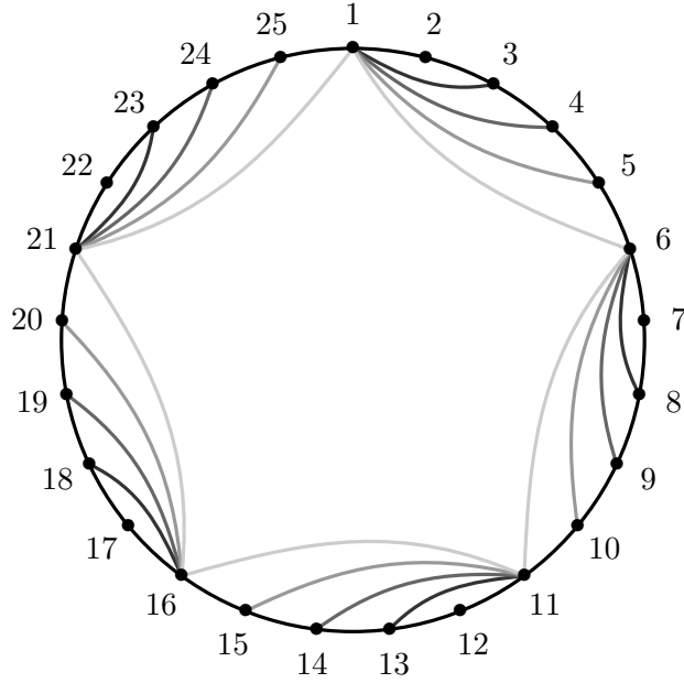
FIGURE 3. A collection of arcs of the icosikaipentagon corresponding to a maximal rigid object in \mathcal{A}_{4,2} .
