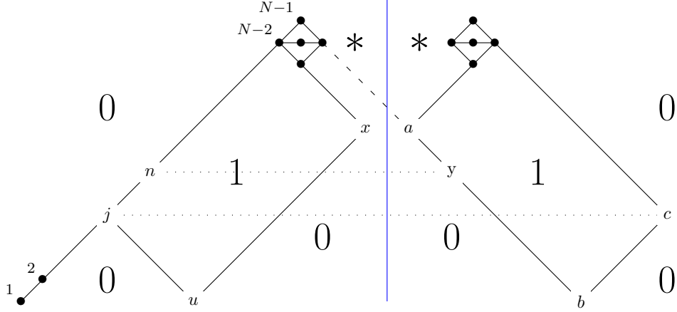
FIGURE 8. Hom-hammocks in the derived category D^b(\mathbb{K}D_N) , N even.
