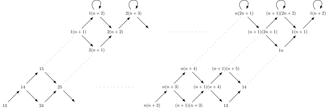
FIGURE 5. The quiver \mathcal{Q}_n
