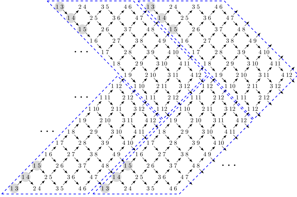
FIGURE 1. A bijection between \frac{2\pi}{5} -periodic collections of arcs of the heptakaidecagon and isomorphism classes of basic objects in \mathcal{A}_{3,2} . The maximal rigid object of Corollary 2.7 is highlighted in grey.
