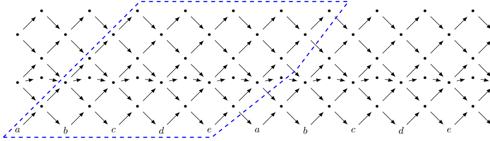
FIGURE 9. The orbit category D^b(\mathbb{K}E_7)/\tau^5 .
