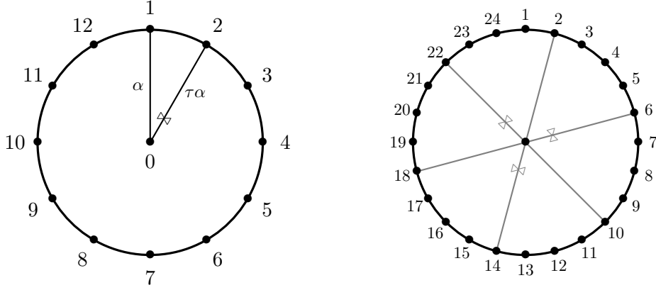
FIGURE 7. Action of \tau on a tagged arc (left) and a non-rigid indecomposable object of \mathcal{D}_{3,3} (right).
